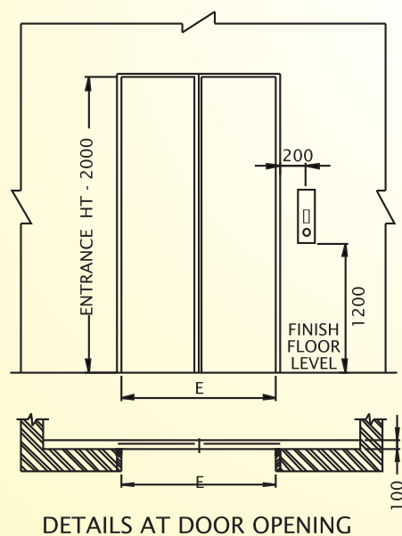
Automatic Centre Opening Doors-Hospital Lifts
